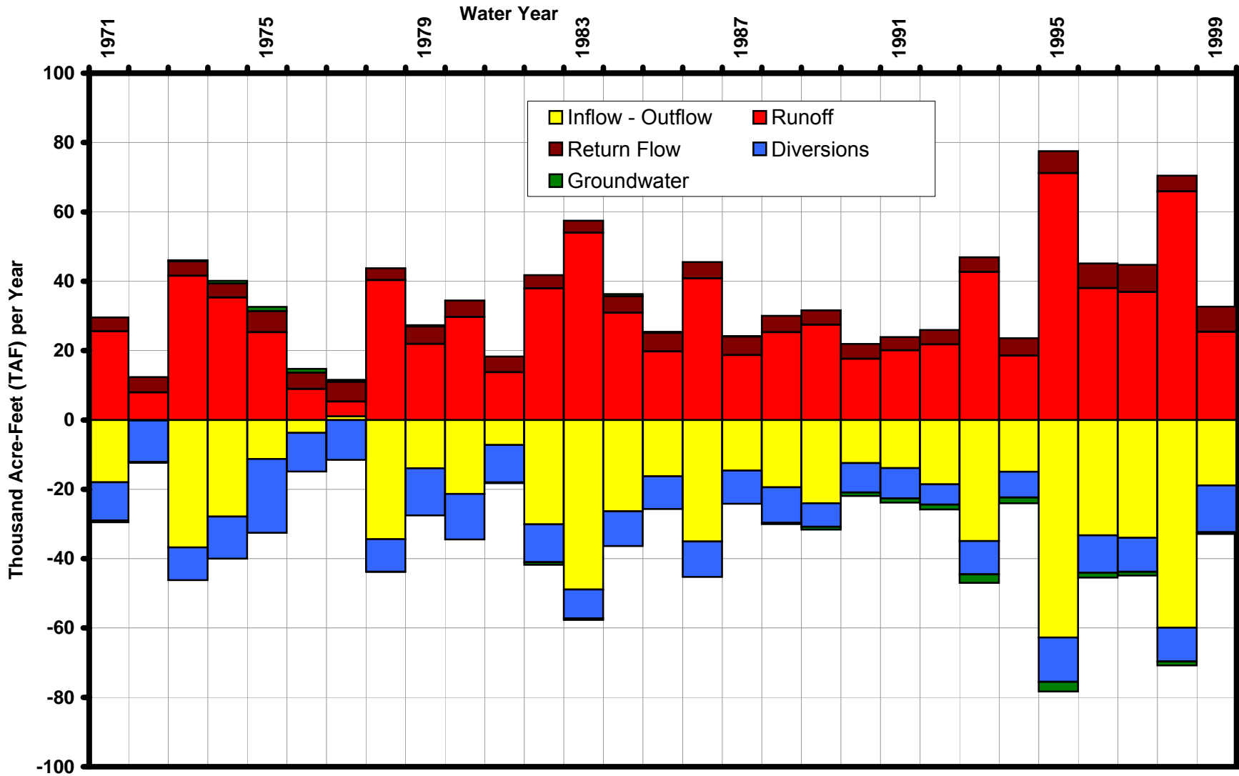
Annual Stream Flow Budget - Subregion 12 - Western Canal
