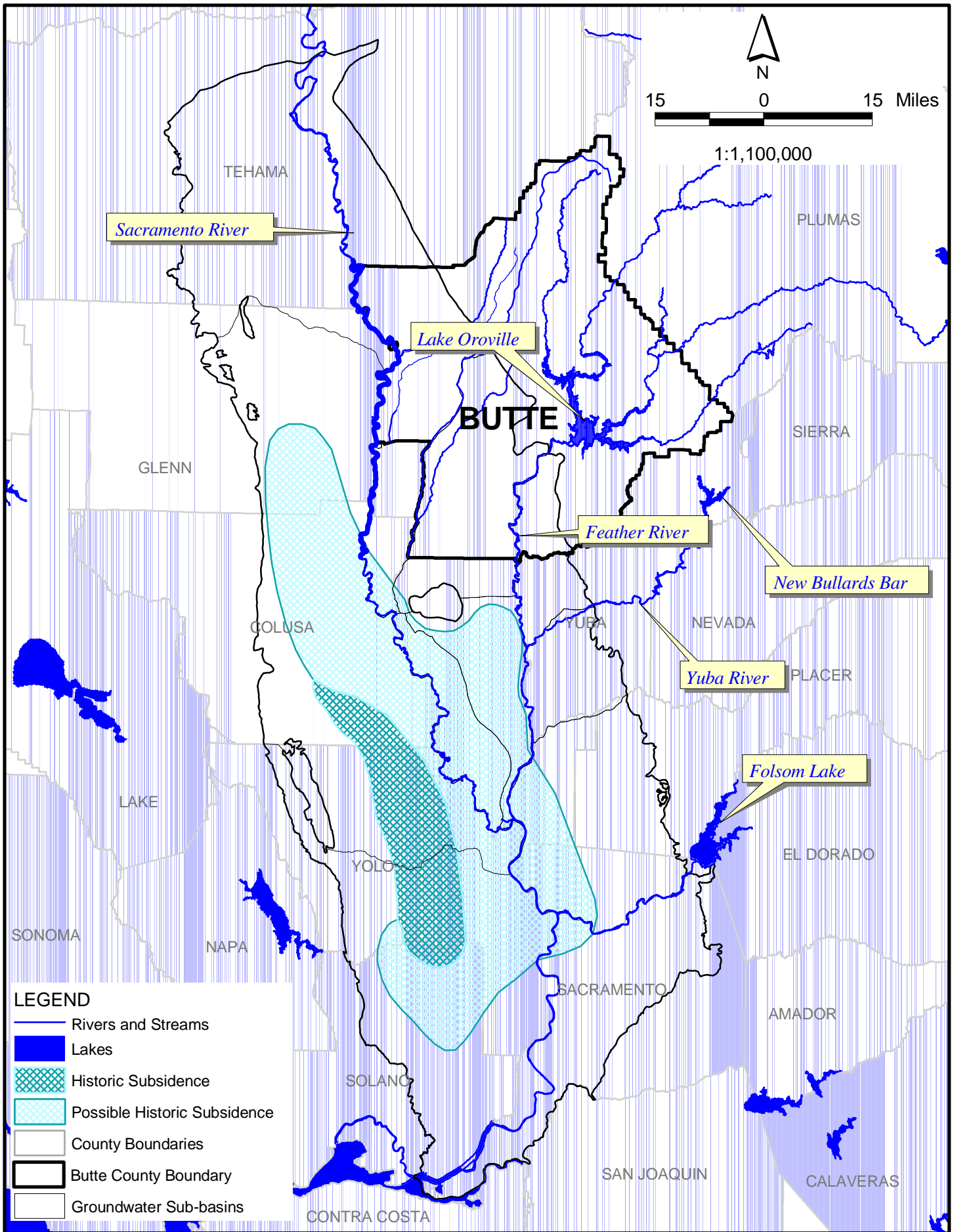
Figure 2-11 Regional Subsidence
