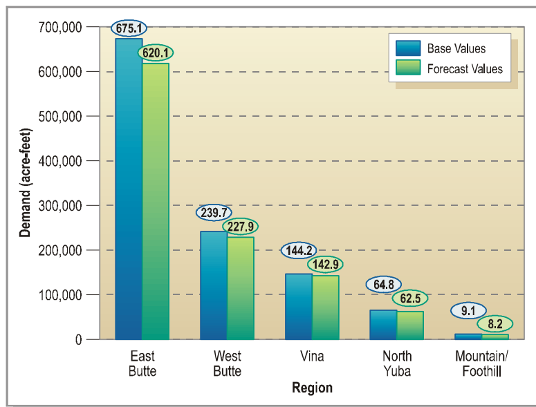
Figure 4-6 Comparison of Total Applied Water Under Base and Combination (Dry Year) Scenarios
